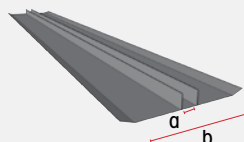
L = 3660mm a = 10mm b = 70mm
