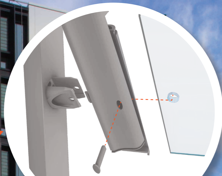
The pin secures the blade to the bearing and clip from inside.
