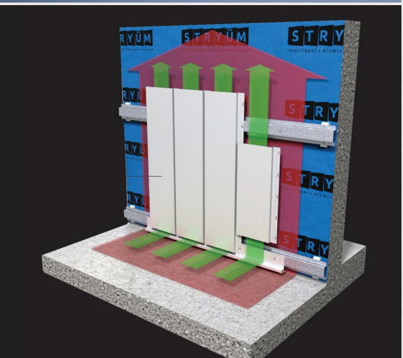
VENTILATED FACADE
