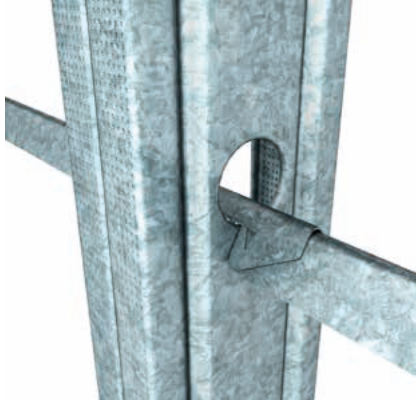
■ OVERLAPPING OF SNAP-LOCK NOGGING WHEN CONTINUOUS
