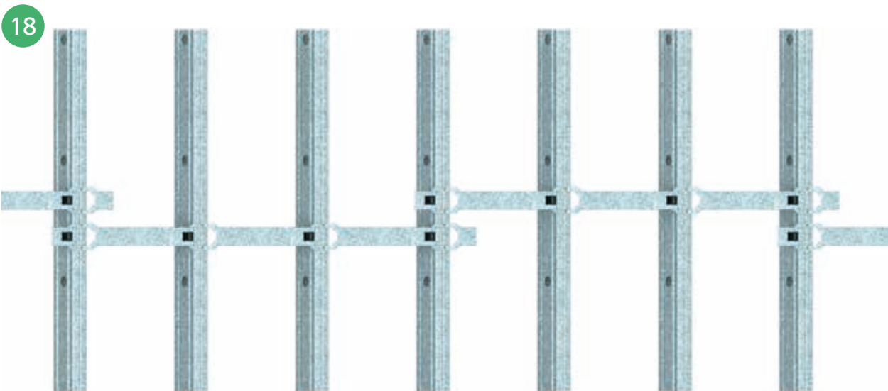
■ FAST-FIX NOGGING CONTINUOUS INSTALLATION
