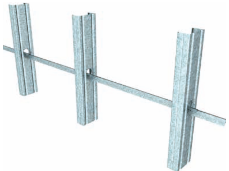
■ CONTINUOUS INSTALLATION OF SNAP-LOCK NOGGING BETWEEN RONDO STEEL STUDS
