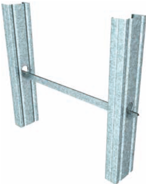
■ SINGLE INSTALLATION OF SNAP-LOCK NOGGING BETWEEN RONDO STEEL STUDS
