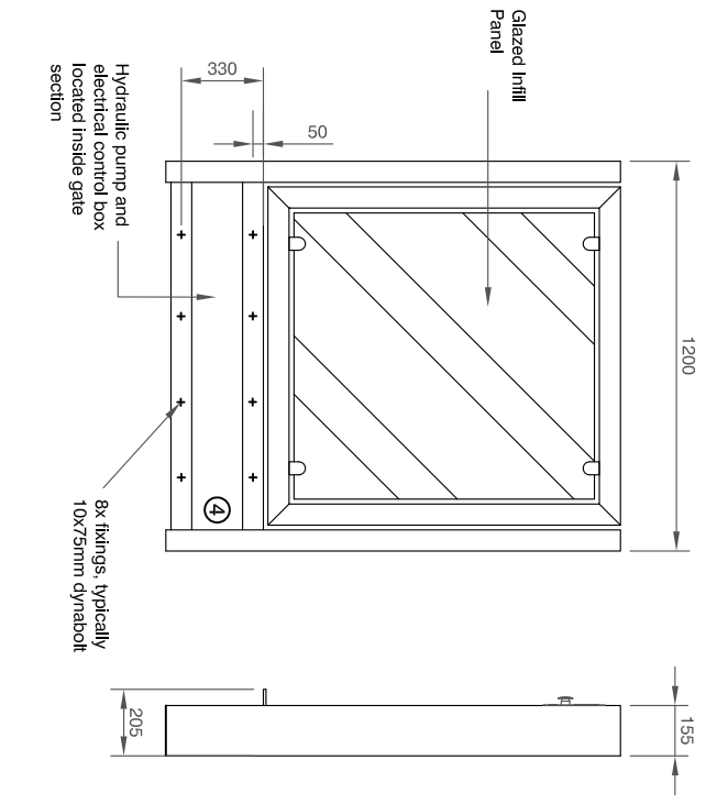
Gate Section Fixing Detail
