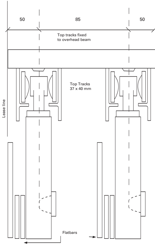
Sectional View
