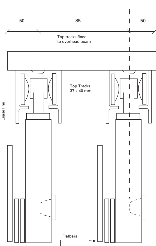
Sectional View
