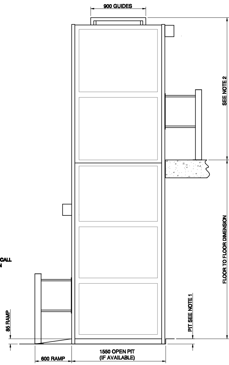
SIDE ELEVATION
