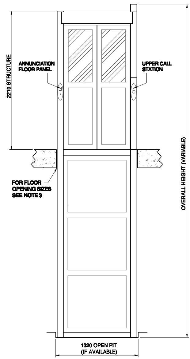
REAR ELEVATION
