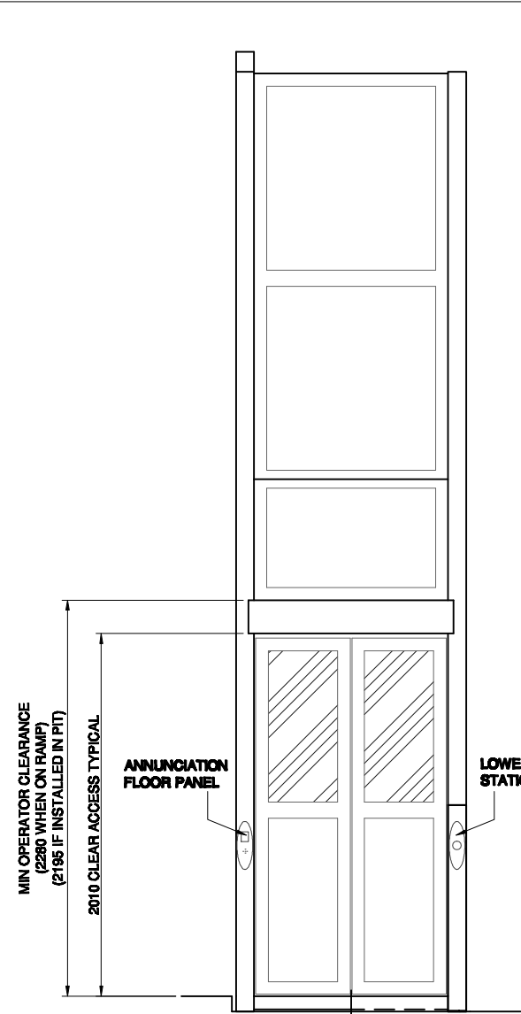
FRONT ELEVATION
