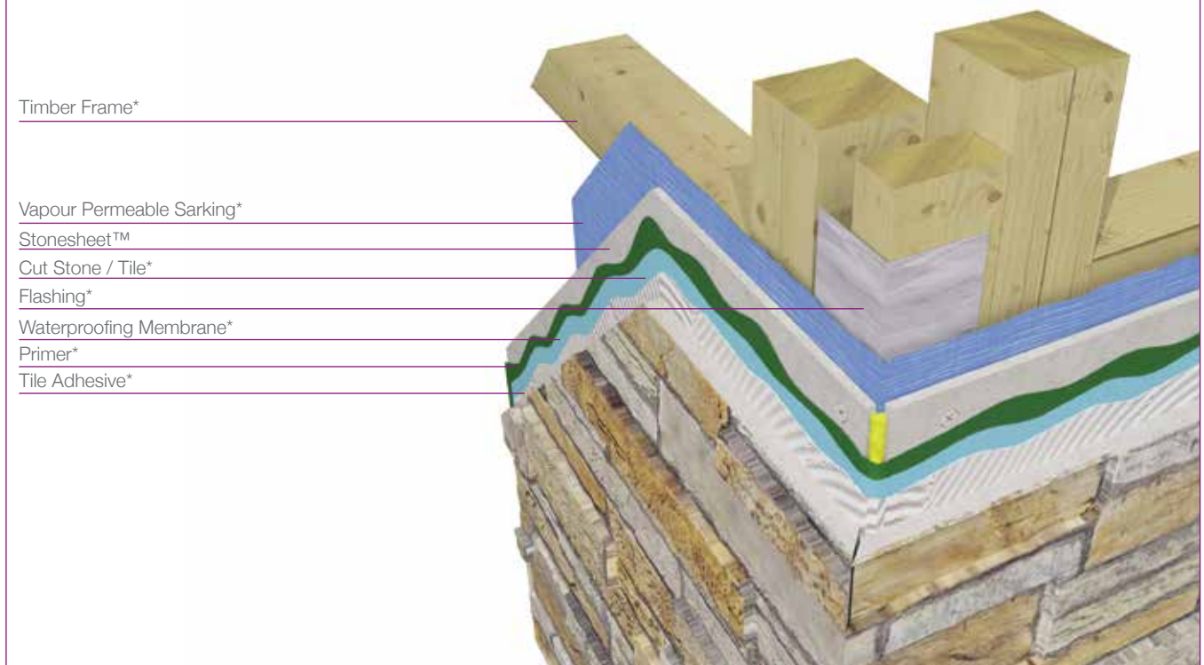
Figure 10 External Corners
