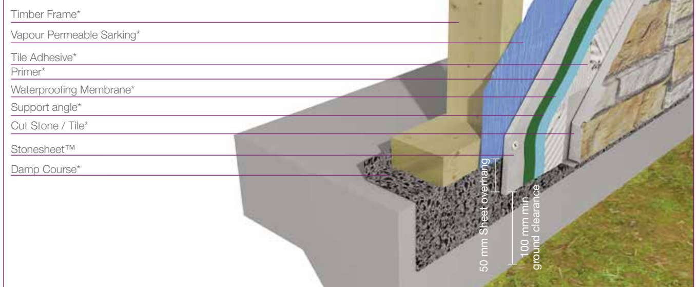
Figure 11 Ground Clearance
