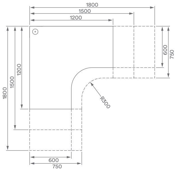
Single Workstation - Internal Radius Worktop
