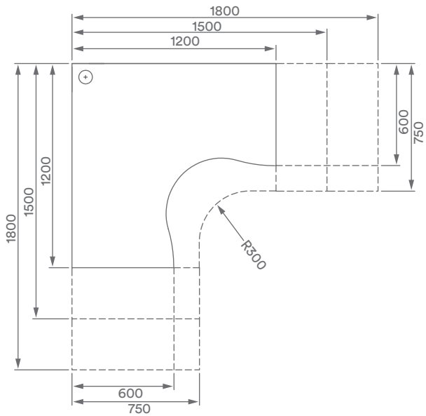
Single Workstation - Internal Freeflow Worktop
