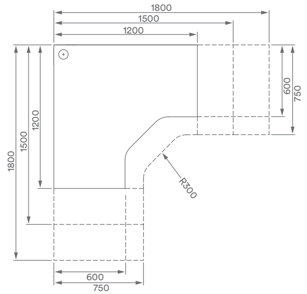
Single Workstation - Internal Splay Worktop
