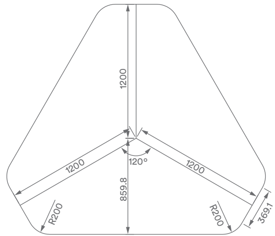
Rounded 120 Degree Worktop
