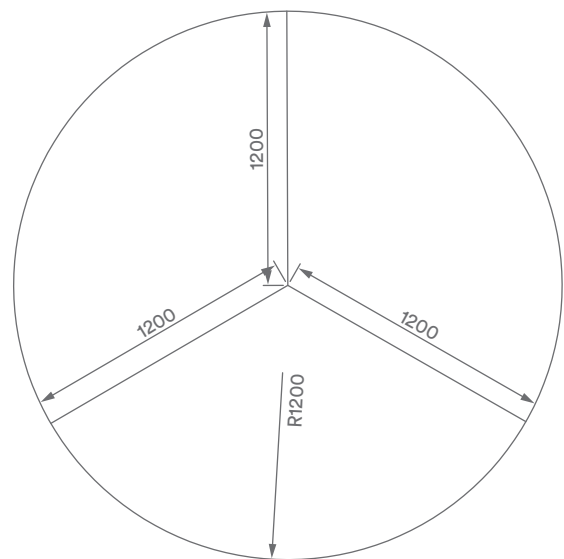
Circular 120 Degree Worktop
